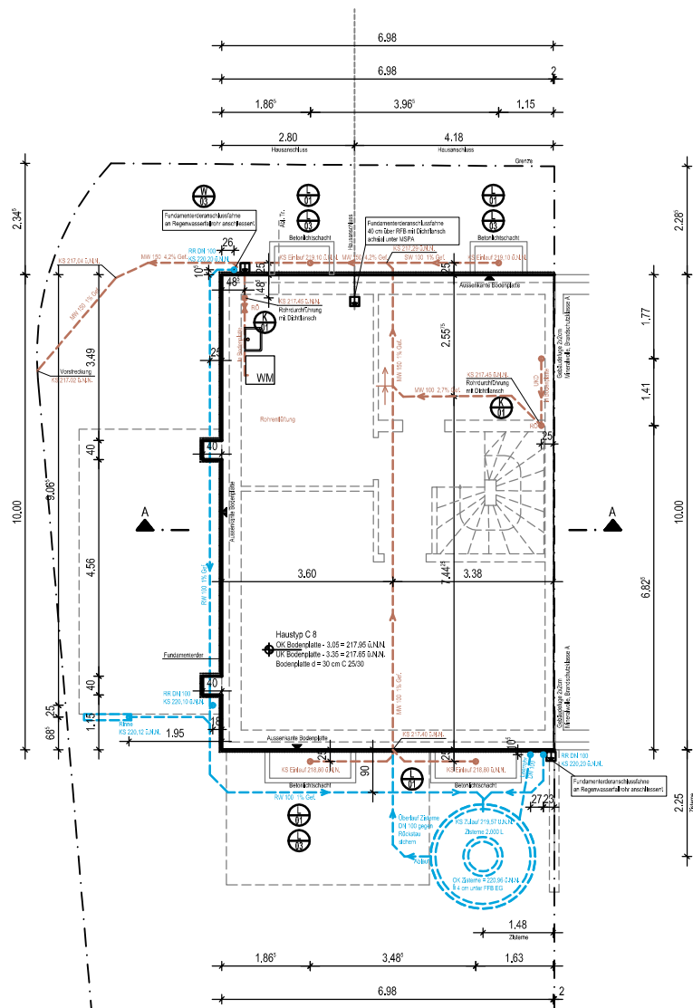
Fundamentplan
